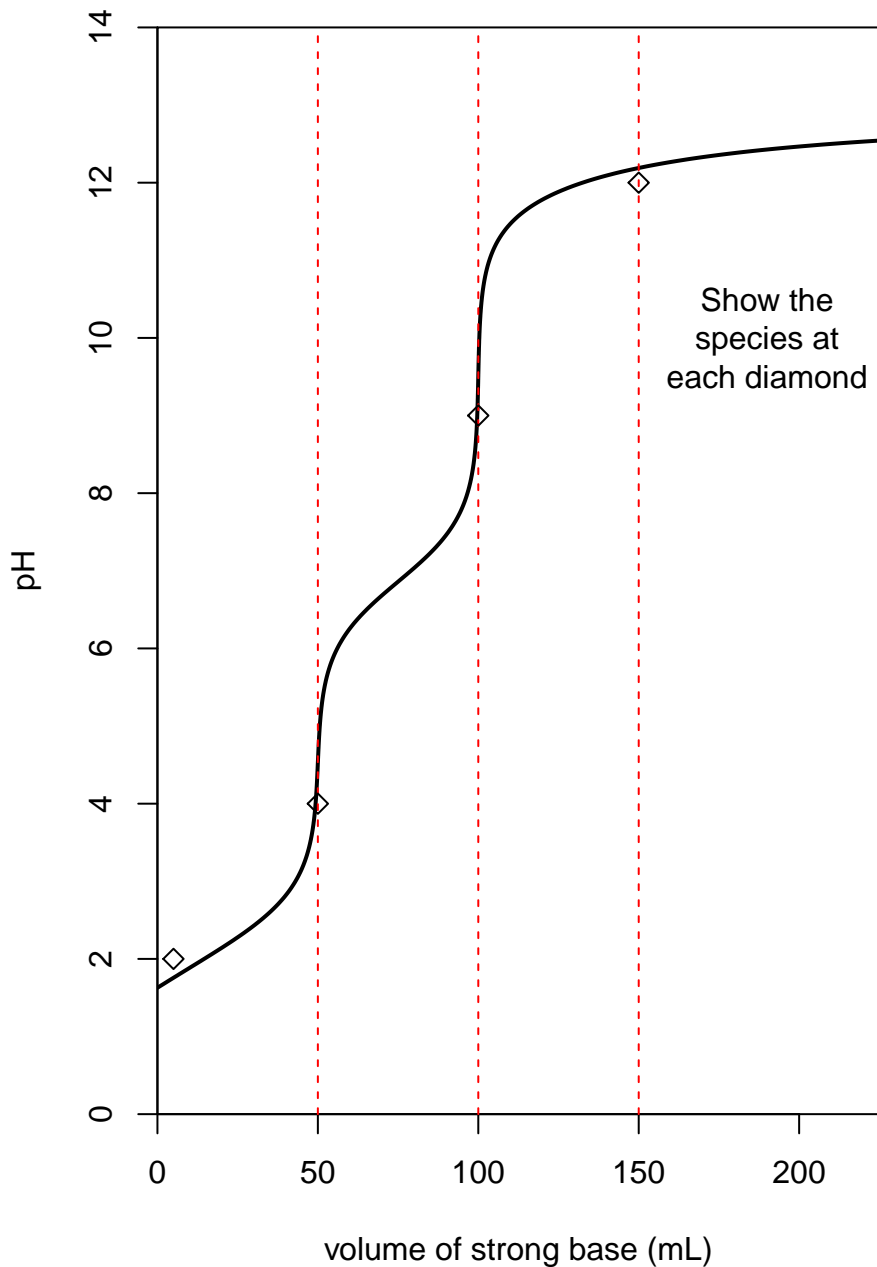
Titration of Phosphoric Acid
